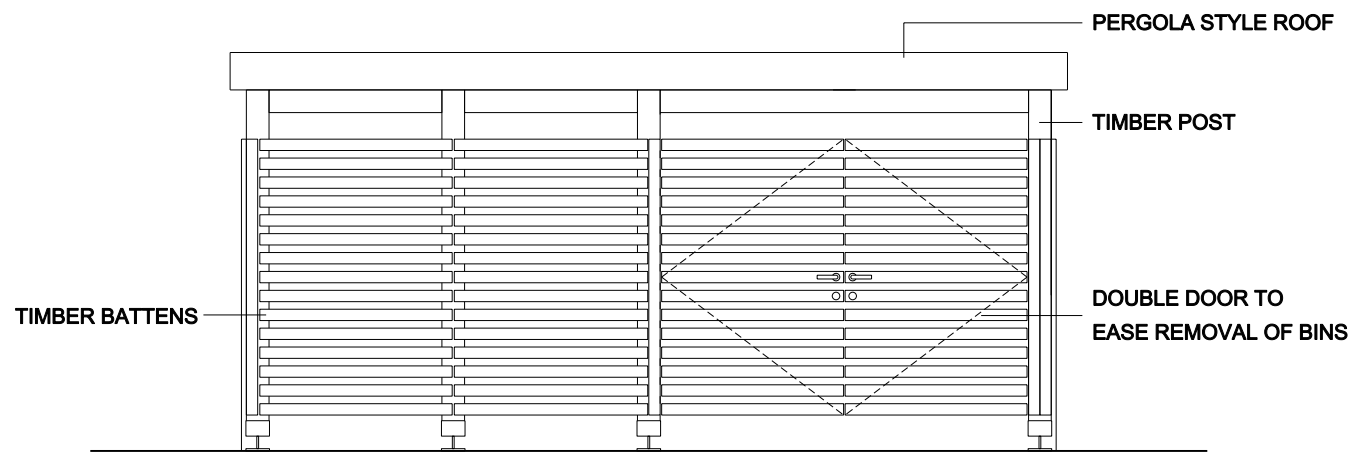
Front Elevation
