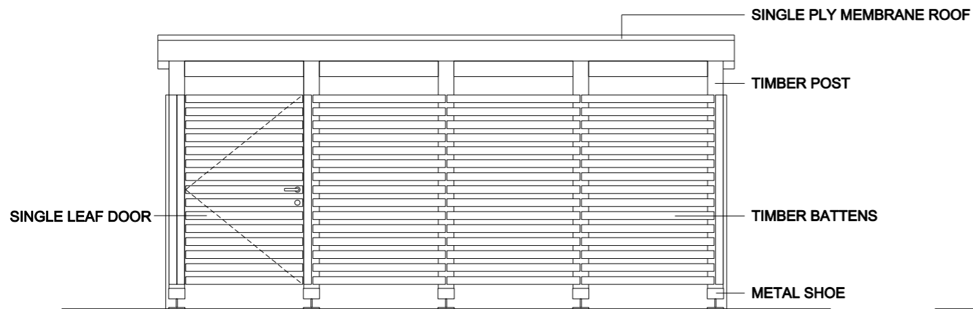
Front Elevation
