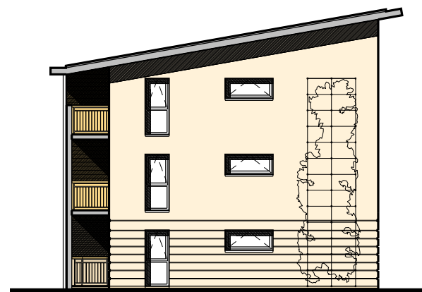
South-East Elevation
