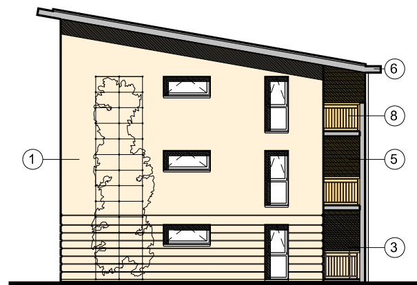
North-West Elevation
